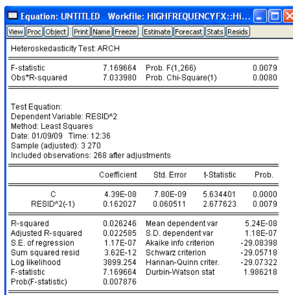
Figure 5.5: ARCH test results
