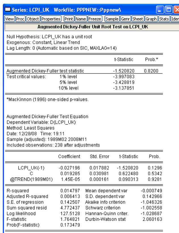
Figure 4.2: Output for the Augmented Dickey-Fuller test
